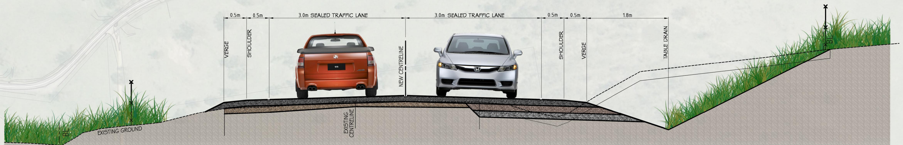
Section 2 detail - Lovely Banks Road Junction to Ringwood Creek Culvert
