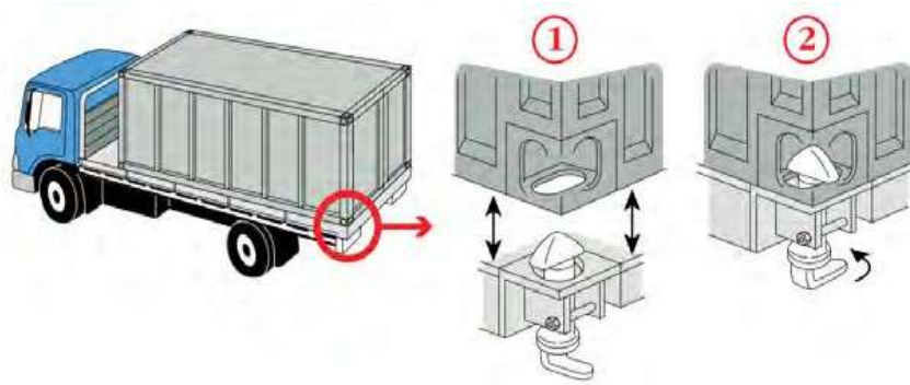
A twist lock used to secure a container.
