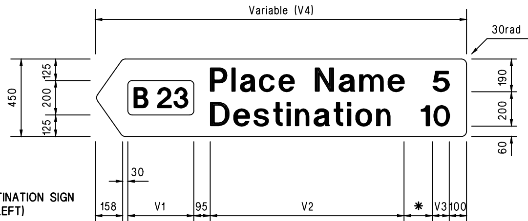
1DL (ONE DESTINATION SIGN POINTING LEFT)
