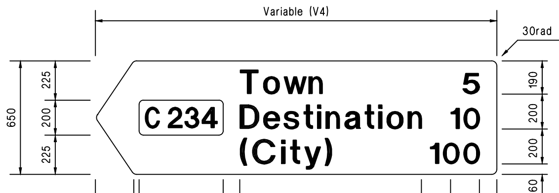
3DL (THREE DESTINATION SIGN POINTING LEFT)
