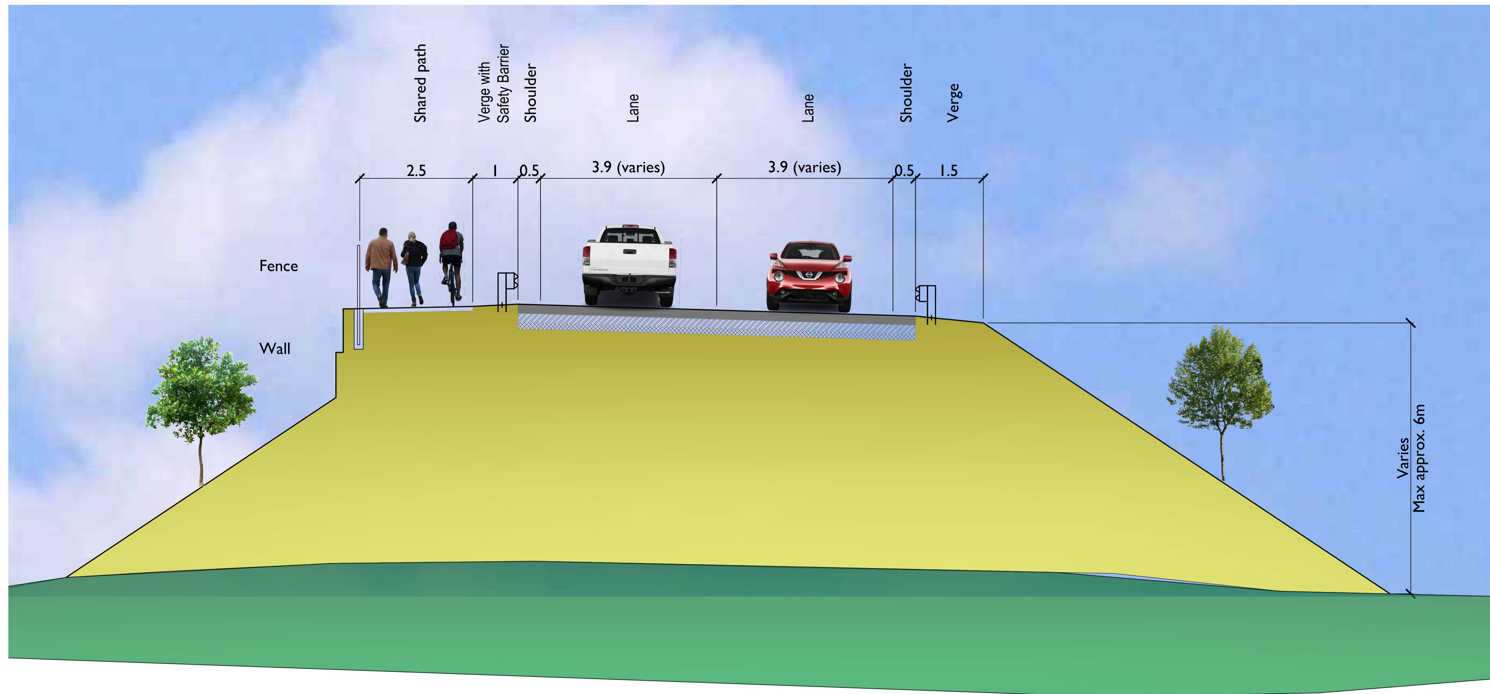
Overpass Typical Section - Leith Road, South of Russell Street
